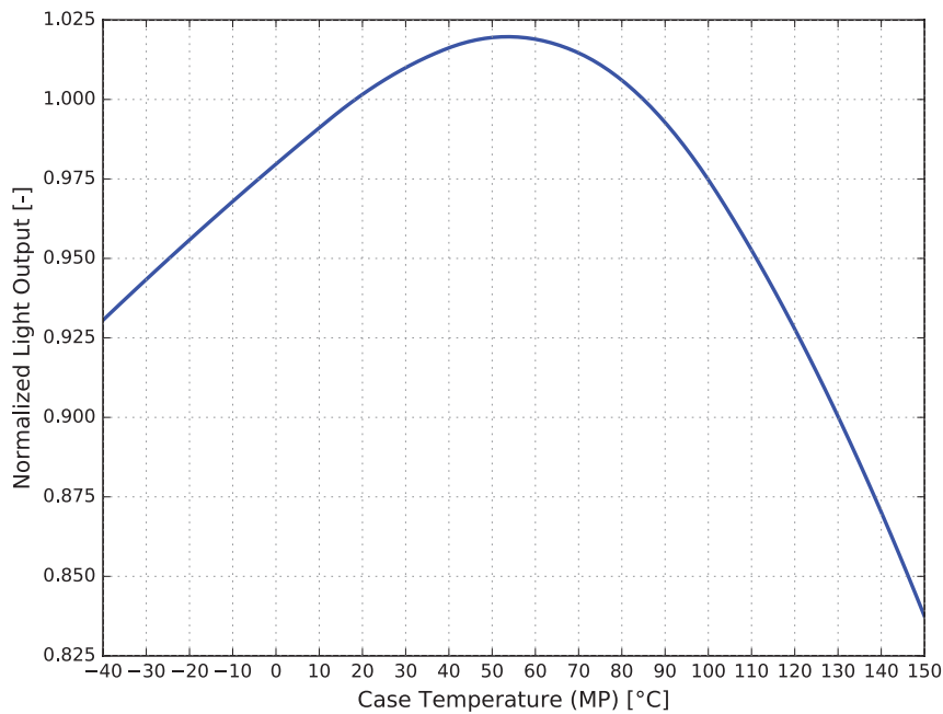
Figure 3a. Typical normalized light output vs. case temperature for LUXEON Altilon Intense Gen2 1x2, 1500 mA MP
