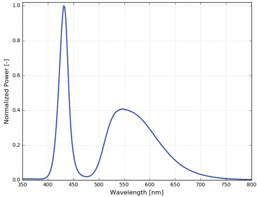
Figure 2. Typical normalized power vs. wavelength for LUXEON Altilon Intense Gen2 1x2, 1500 mA MP, T_c = 85\text{ }^\circ\text{C}
