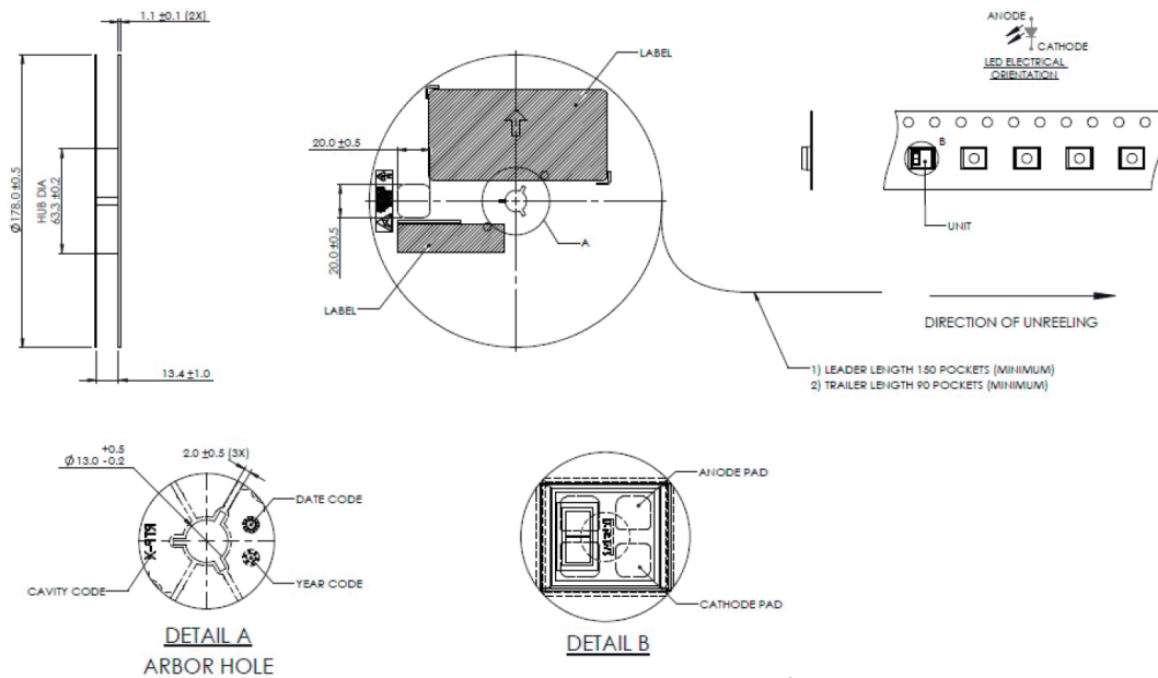
Figure 12. Reel dimensions for LUXEON Altilon Intense Gen2 1x2
