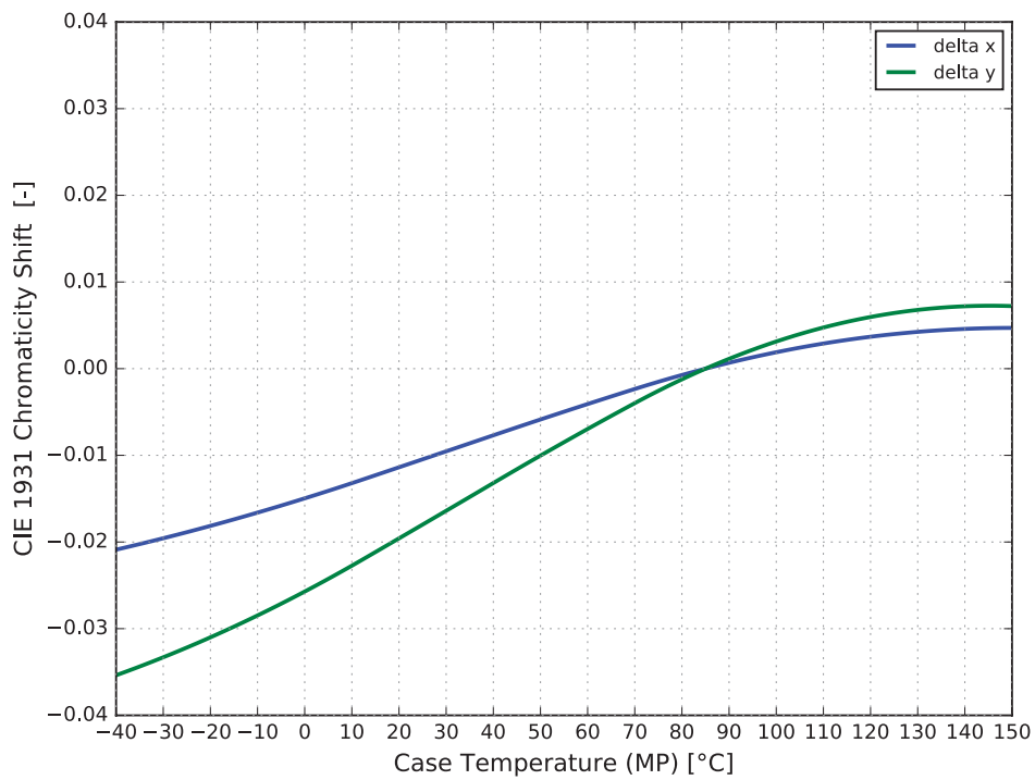
Figure 5a. Typical color shift in CIE 1931 x and y coordinates vs. case temperature for LUXEON Altilon Intense Gen2 1x2
