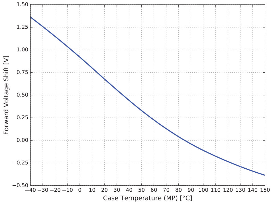
Figure 4b. Typical forward voltage vs. case temperature for LUXEON Altilon Intense Gen2 1x2, 1500 mA MP
