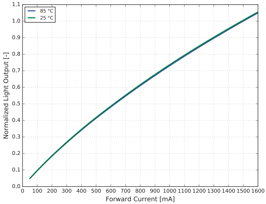
Figure 3b. Typical normalized light output vs. forward current for LUXEON Altilon Intense Gen2 1x2, MP, 25 °C and T_c = 85 °C
