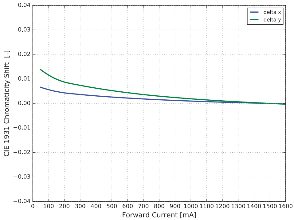
Figure 5b. Typical color shift in CIE 1931 x and y coordinates vs. forward current for LUXEON Altilon Intense Gen2 1x2, T_c = 85\text{ }^\circ\text{C}
