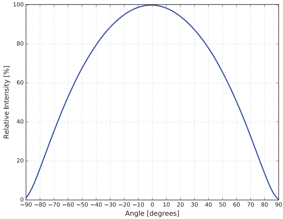
Figure 6. Typical radiation pattern for LUXEON Altilon Intense Gen2 1x2
