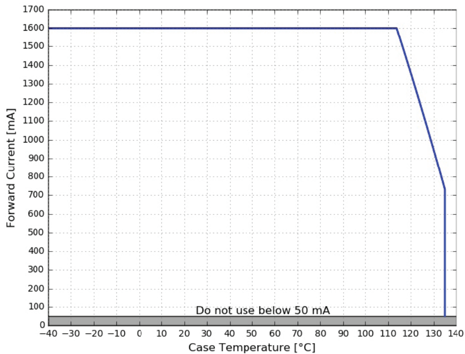
Figure 7. Maximum forward current vs. case temperature for LUXEON Altilon Intense Gen 2 1x2
