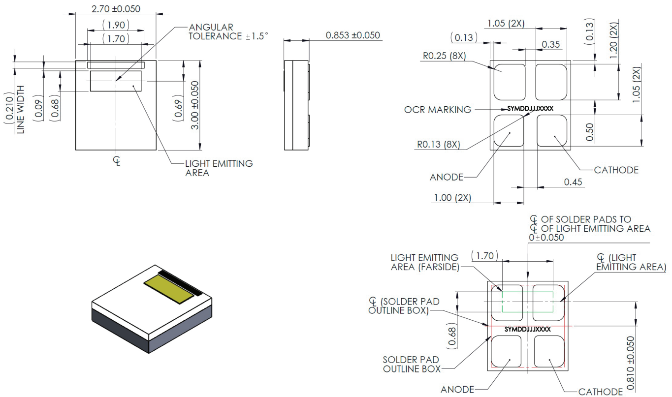
Figure 10. Mechanical dimensions for LUXEON Altilon Intense Gen2 1x2
