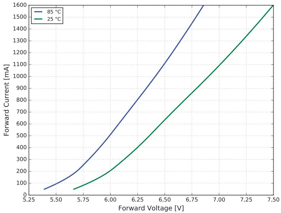
Figure 4a. Typical forward current vs. forward voltage for LUXEON Altilon Intense Gen2 1x2, MP, 25 °C and T_c = 85 °C
