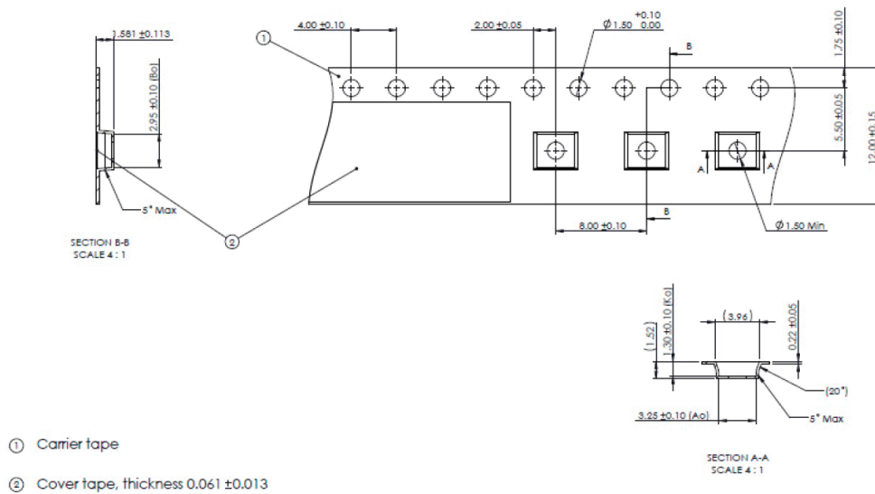
Figure 11. Pocket tape dimensions for LUXEON Altilon Intense Gen2 1x2
