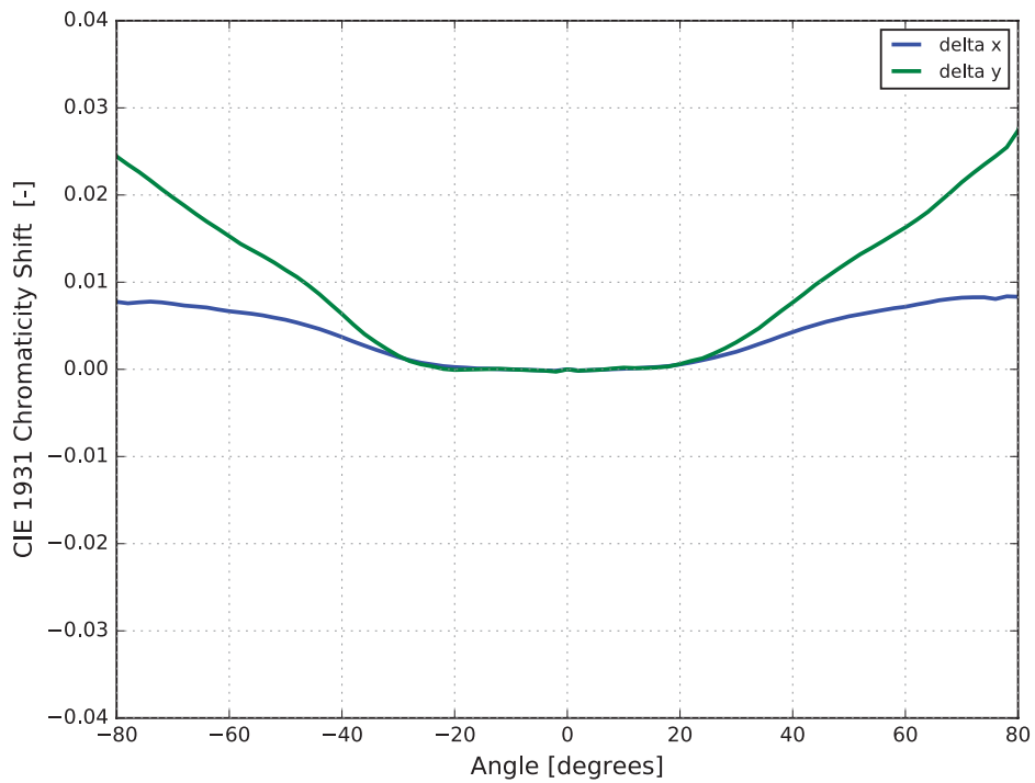
Figure 5c. Typical color shift in CIE 1931 x and y coordinates vs. angle for LUXEON Altilon Intense Gen2 1x2
