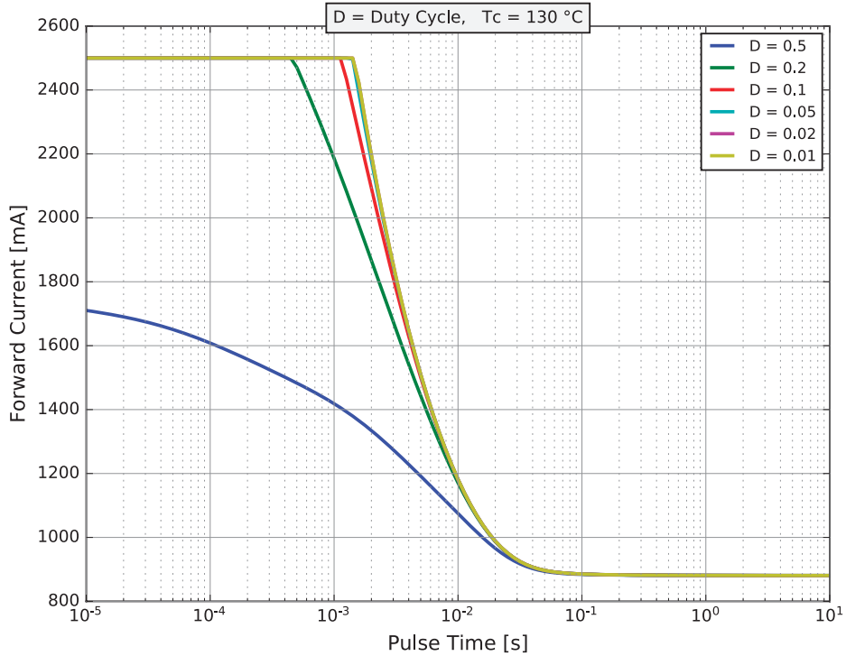
Figure 8. Permissible pulse handling capability for LUXEON Altilon Intense Gen2 1x2
